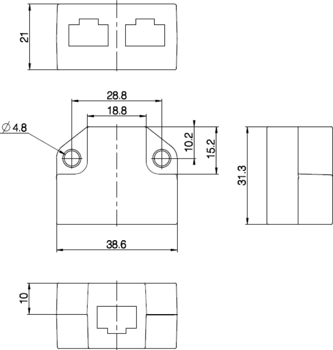
T-splitter
