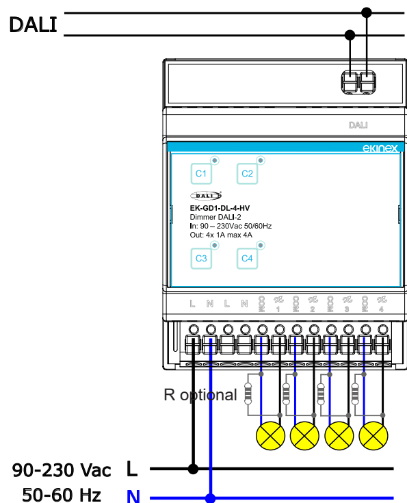
Installation diagram with outputs with separate COM pole connection
