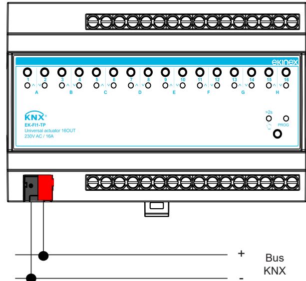
e KNX bus connection
