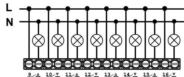
f Output connection (EK-F11-TP used as 16-channel binary output)
