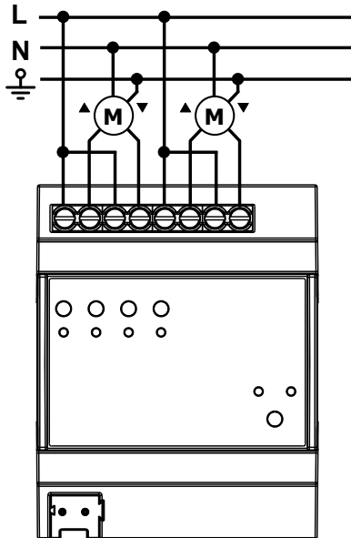
g Output connection (EK-FH1-TP used as 2-channel actuator for drive control).
