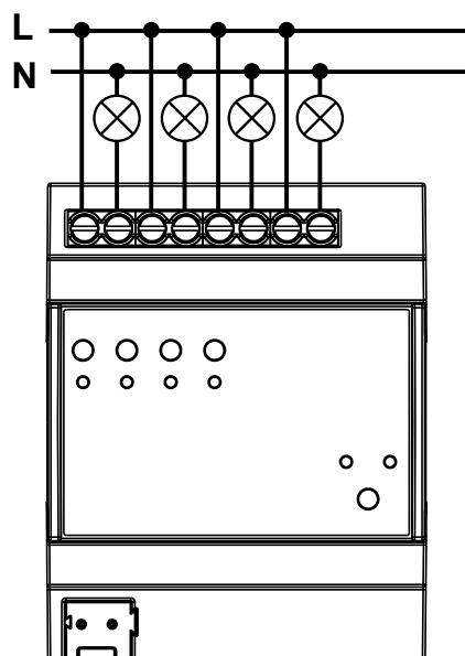
f Output connection (EK-FH1-TP used as 4-channel binary output)
