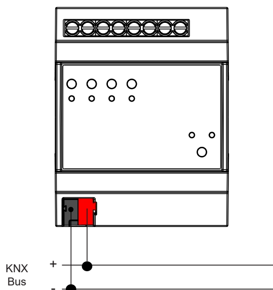
e KNX bus connection
