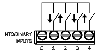
i Connection as 2 pairs of inputs (e.g., coupled buttons for controlling dimmers or motorized drives). Also connect the outputs as in (g).
