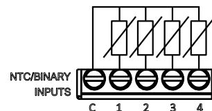
j Connection as 4 individually configurable inputs for passive temperature probes (NTC 10 kΩ at 25 °C).
