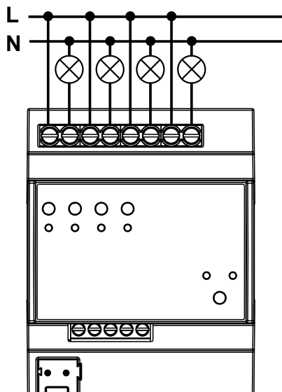
f Connection of the loads (device EK-FH1-TP-I used as 4-fold binary output).
