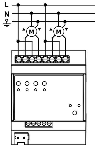
g Connection of the loads (device EK-FH1-TP-I used as 2-fold blind actuator).
