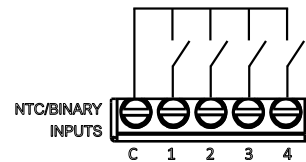
h Connection as 4 independent inputs (connection of traditional switches or buttons dedicated to the on/off control of utilities).
