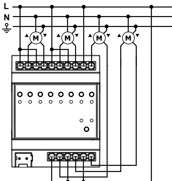
g Connection of the loads (device EK-FG1-TP used as 4-fold blind actuator).
