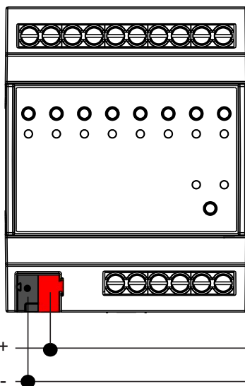
e KNX bus line connection
