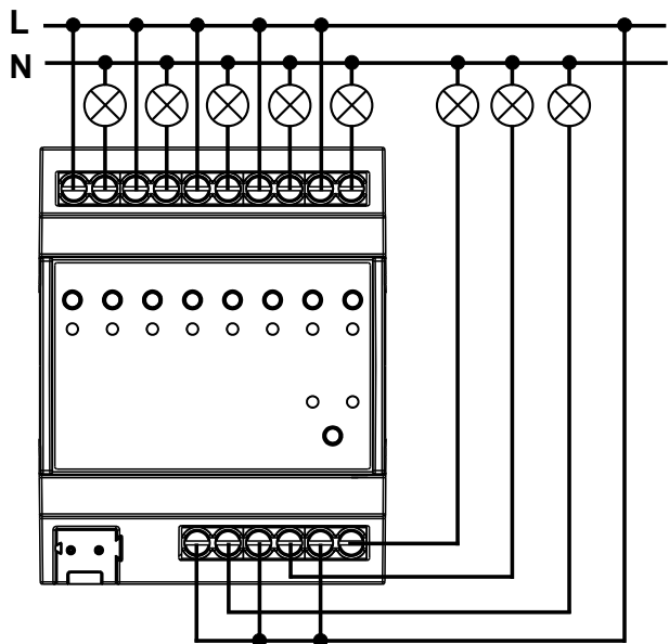
f Connection of the loads (device EK-FG1-TP used as 8-fold binary output).
