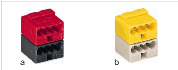
a) Terminal block for conductor pair 1 (black/red) b) Terminal block for conductor pair 1 (white/yellow)
