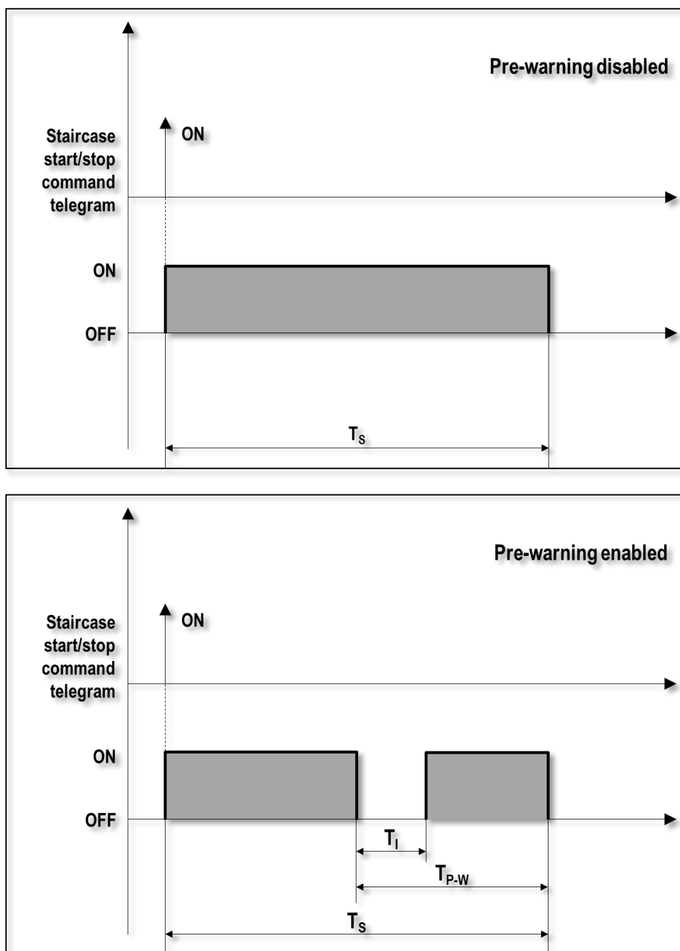
Fig. 6 - Pre-warning feature
