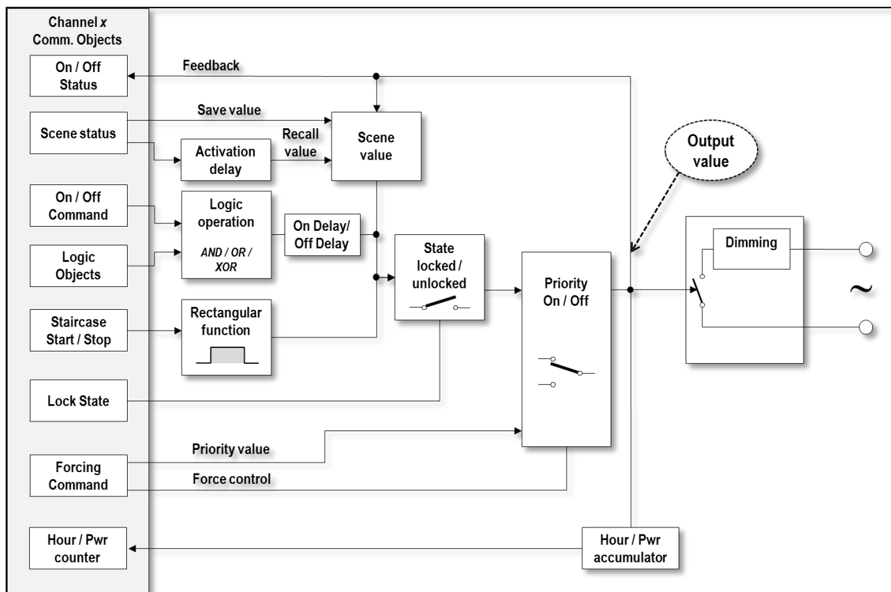
Fig. 2 - Functional blocks
