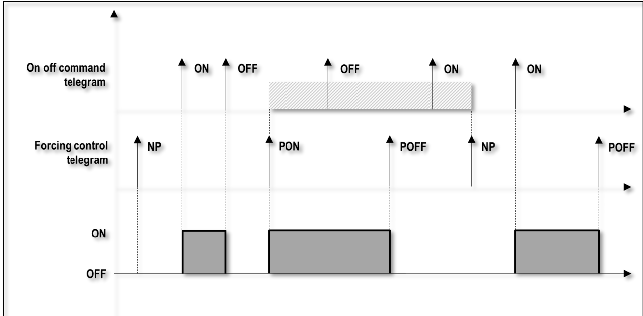
Fig. 12 - Forcing function
