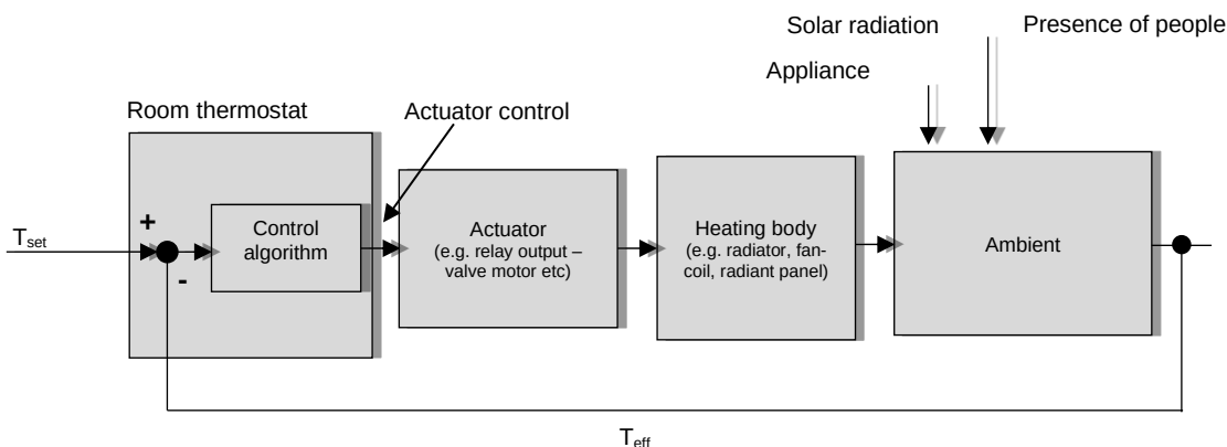
Figure 31 - Generic control system for room temperature regulation
