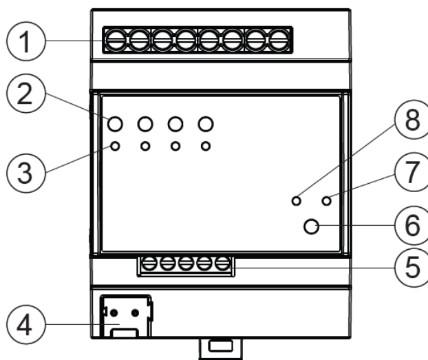
Figure 3 - Switching, display and connection elements for EK-FH1-TP-I
