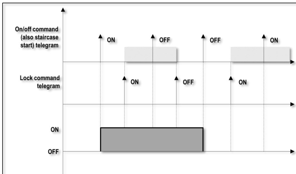
Figure 12- Lock function
