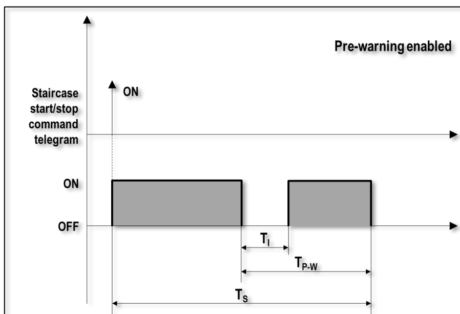
Figure 11 - Pre-warning feature (enabled)
