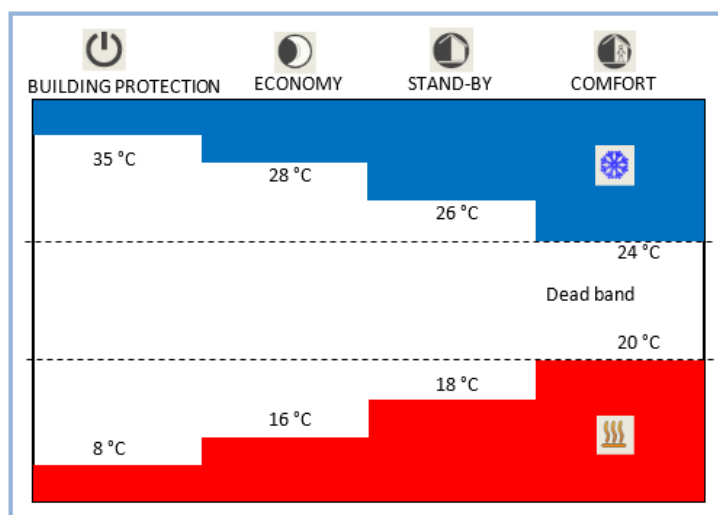
Figure 40 - Dead zone and example of consistently distributed setpoint values
