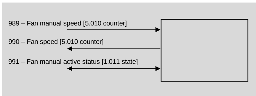
Figure 44 - Remote fan speed adjustment
