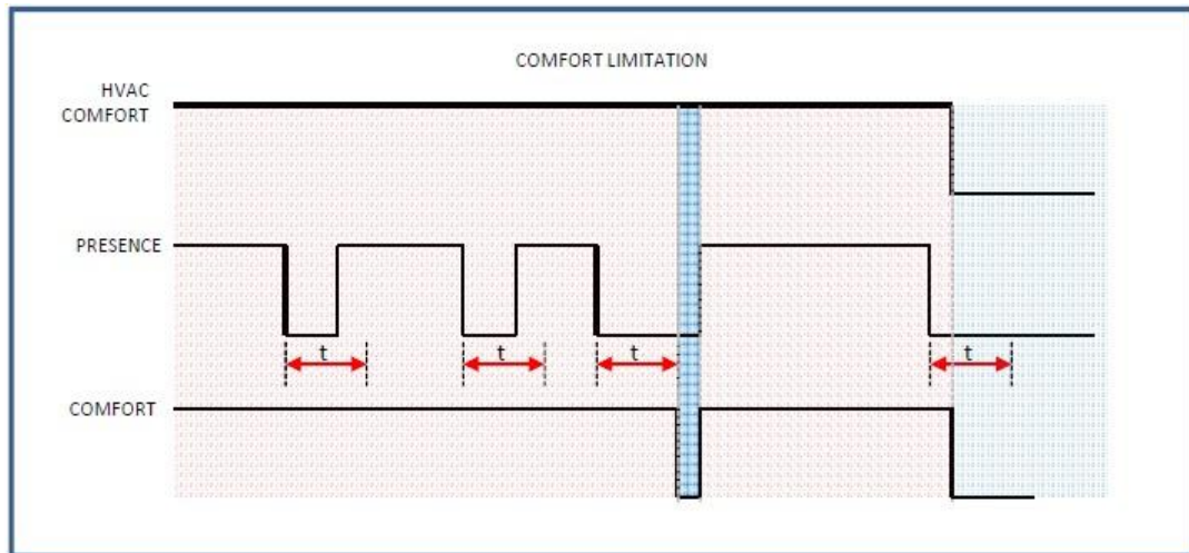
Figure 37 - Comfort limitation
