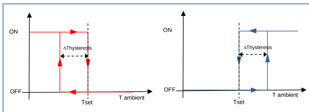
Figure 32 - Temperature control with hysteresis
