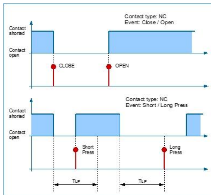
Figure 22 - time diagrams for NC (Normally Closed) mode
