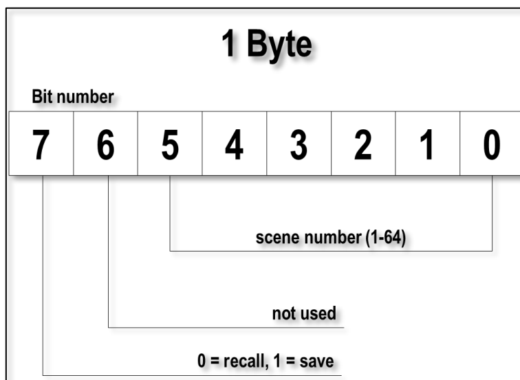
Figure 15 - Scene store / recall command code
