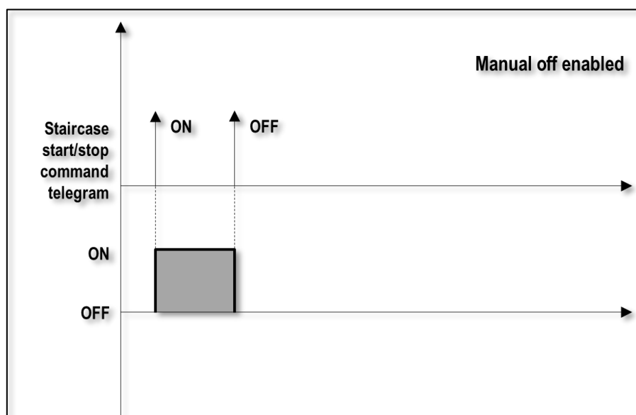
Figure 7 - Manual Off feature (enabled)
