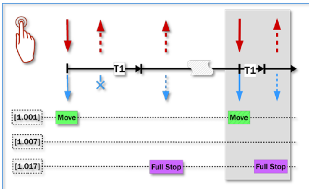
Figure 25 - Shutter mode command sequence
