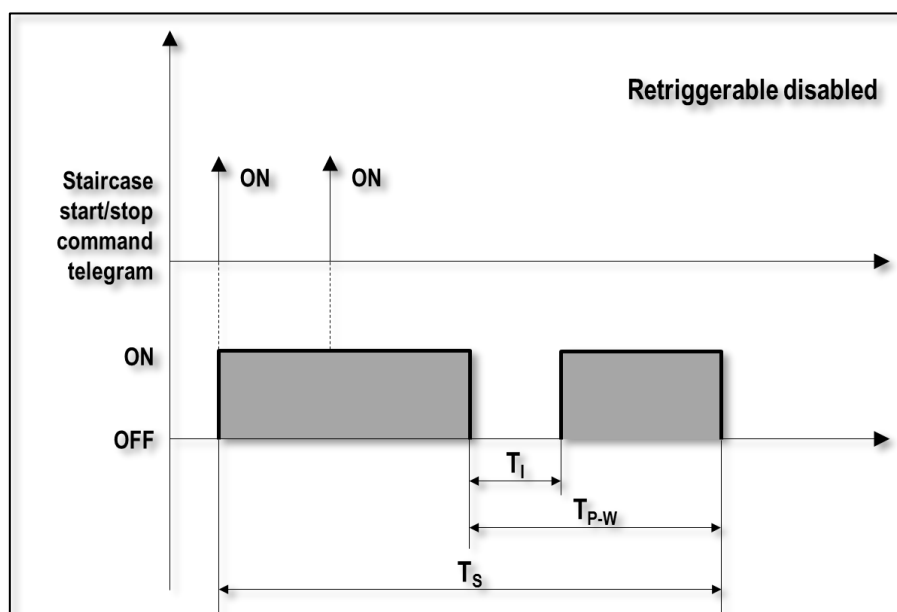
Figure 8 - Retrigger feature (disabled)
