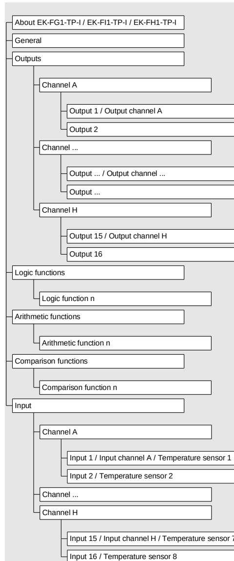
Figure 38 - ETS application program parameters
