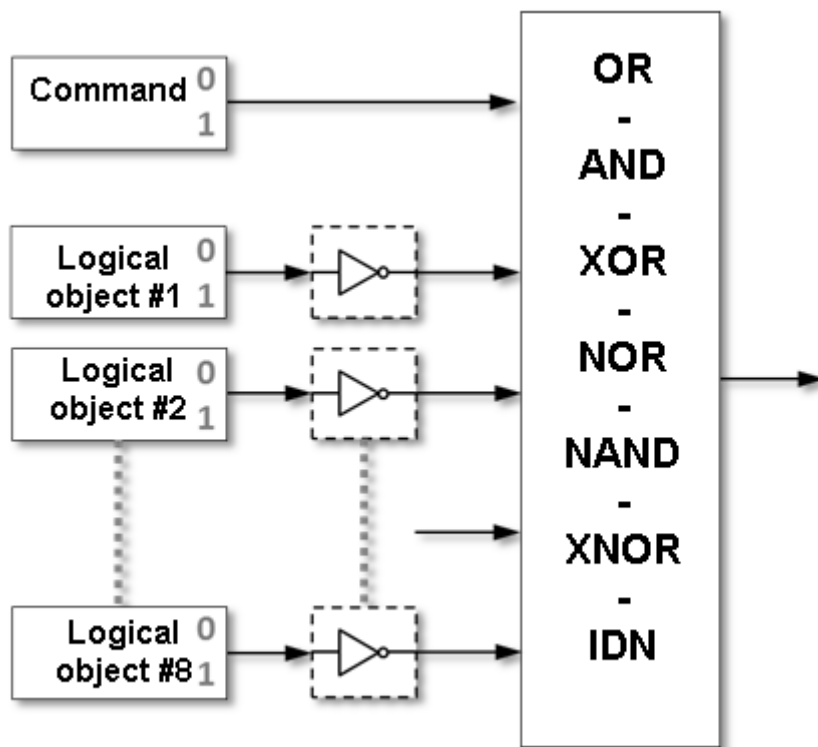
Figure 27 - Logical combination function
