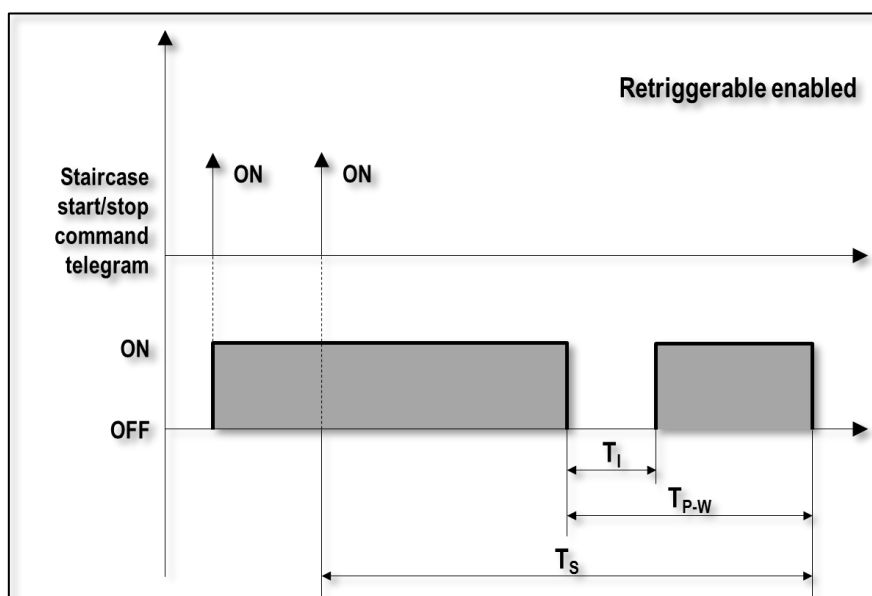
Figure 9 - Retrigger feature (enabled)
