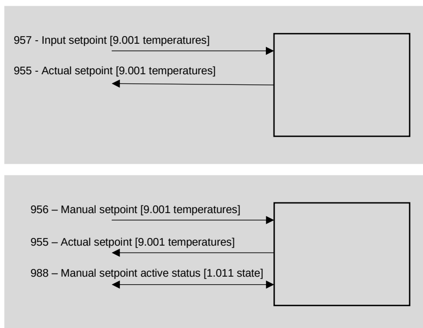
Figure 42 - Manual setpoint modification
