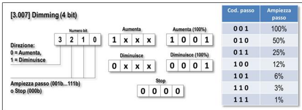
Figure 23 - Dimming communication object
