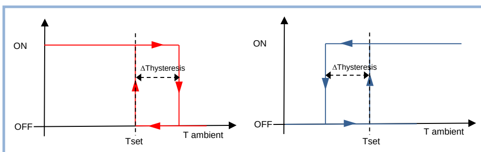
Figure 33 - Two-points temperature regulation
