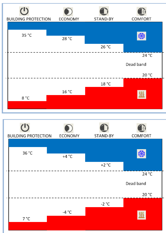
Figure 35 - Automatic switch-over, based on room temperature
