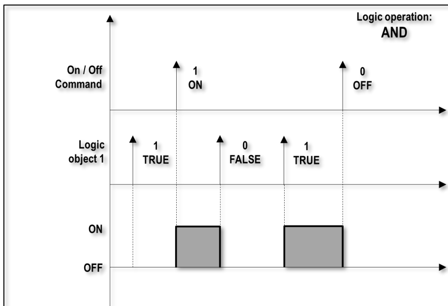
Figure 29 - Logic function AND
