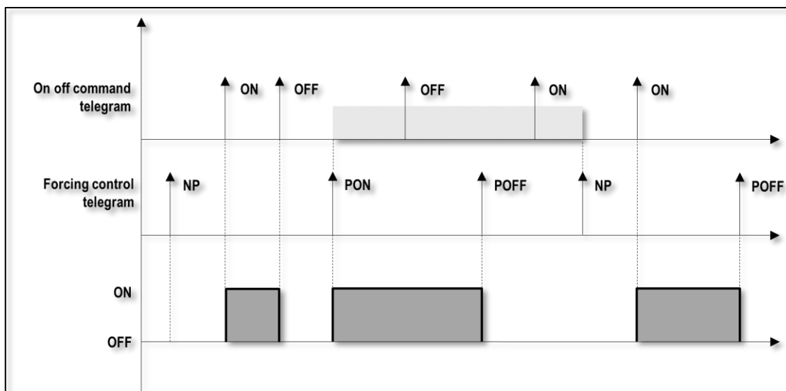
Figure 13 - Forcing function
