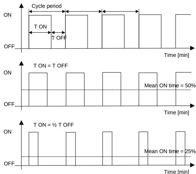
Figure 34 - PWM regulation scheme
