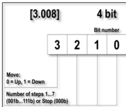
Figure 18 - Shutter control with dimming
