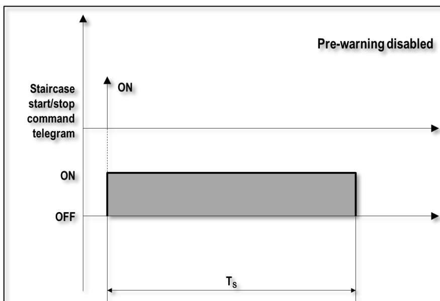
Figure 10 - Pre-warning feature (disabled)
