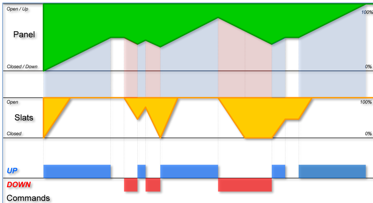
Figure 19 - Venetian blind control diagram
