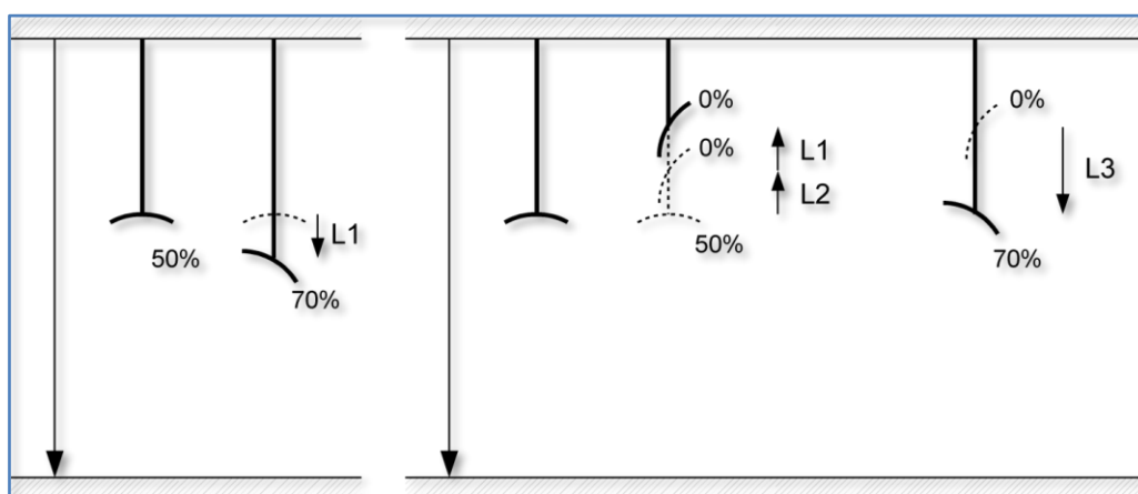
Figure 20 - Compensation for slat movement
