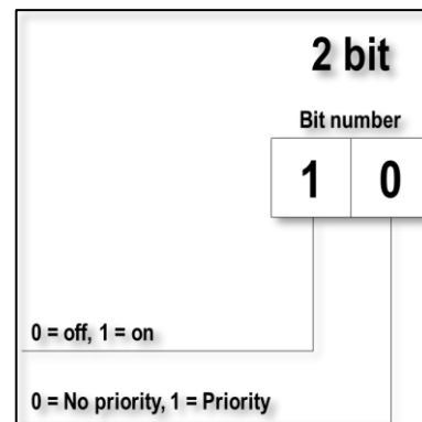
Figure 14 - Force command bits
