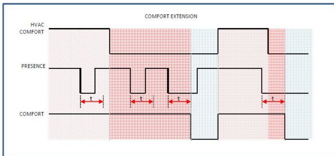
Figure 36 - Comfort extension
