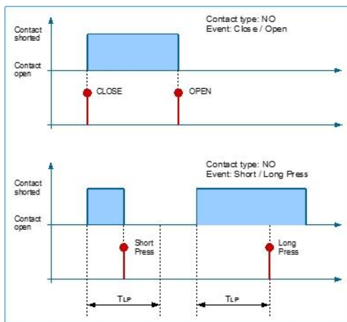
Figure 21 - time diagrams for Normally Open (NO) mode
