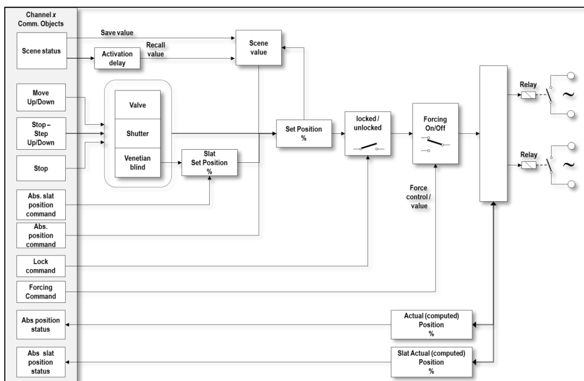
Figure 17 - Functional blocks – Coupled mode (referred to a single output)
