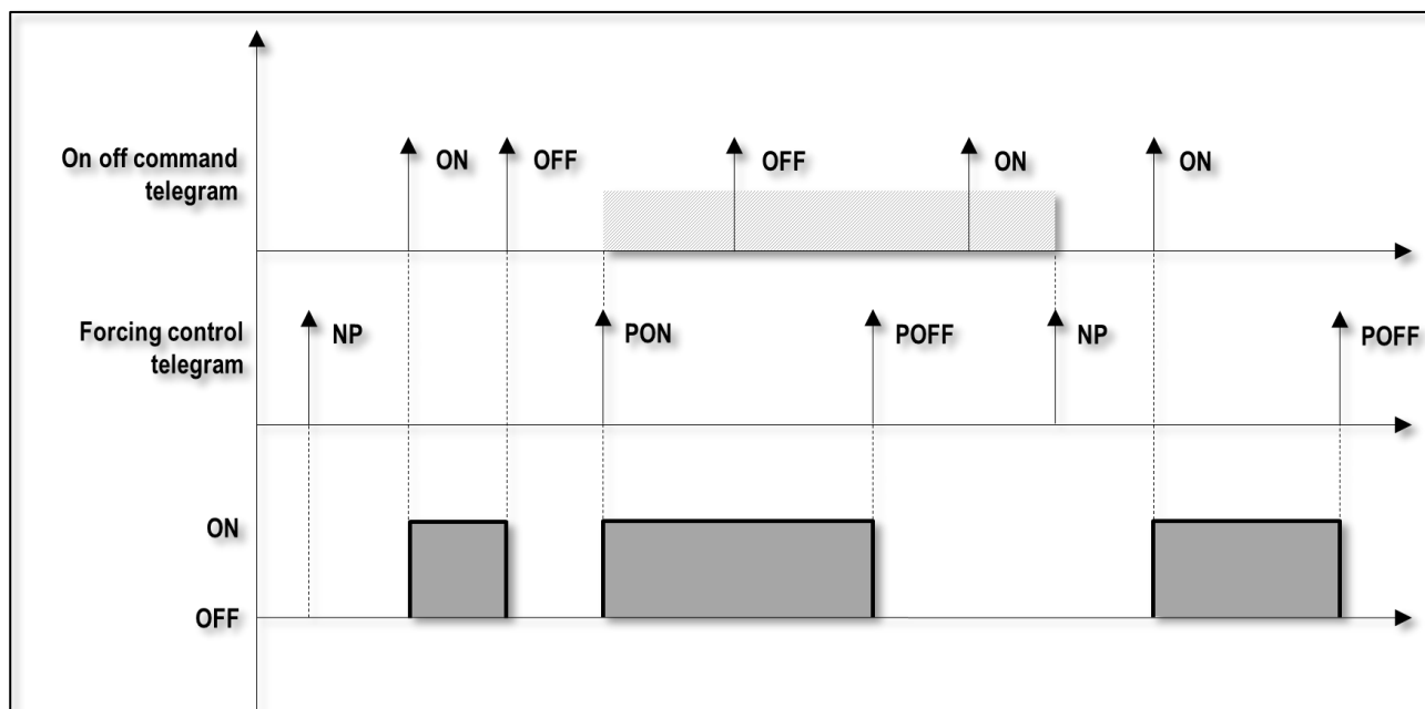
Fig. 12 - Forcing function
