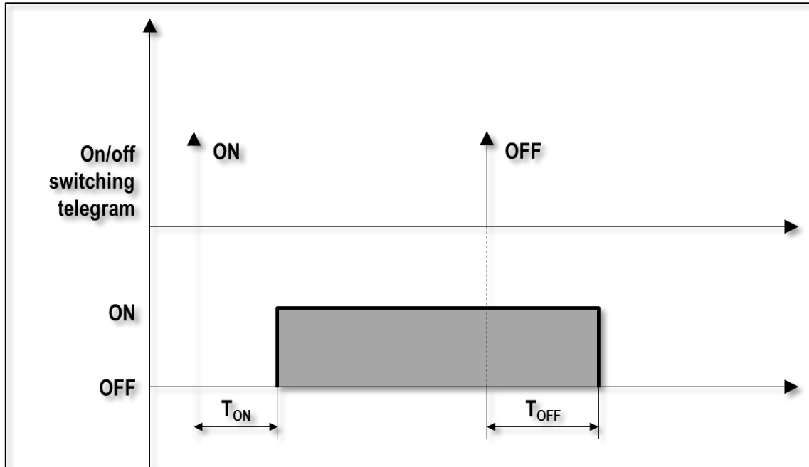
Fig. 3 - Time delay
