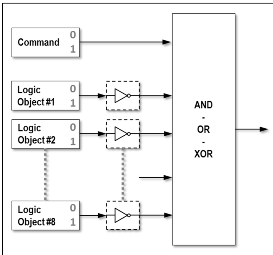
Fig. 7 - Logic functions
