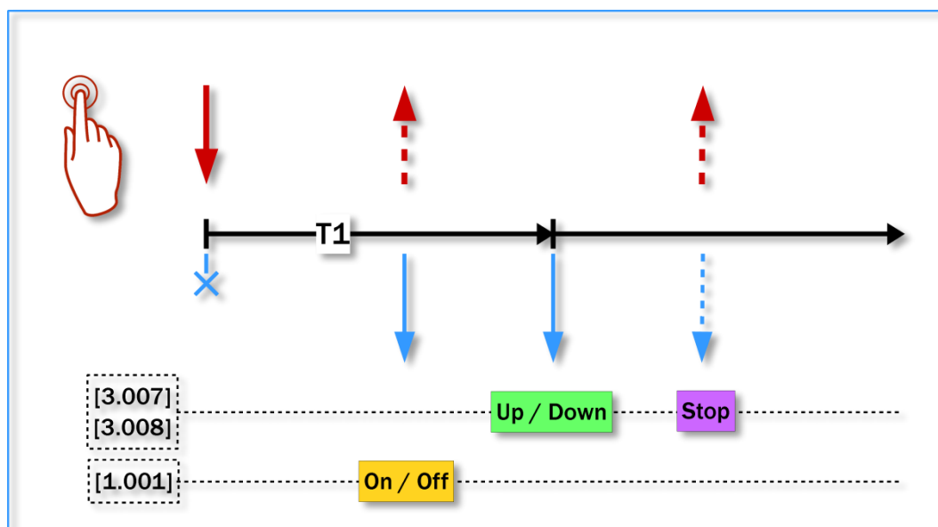
Figure 4 - Dimmer mode command sequence
