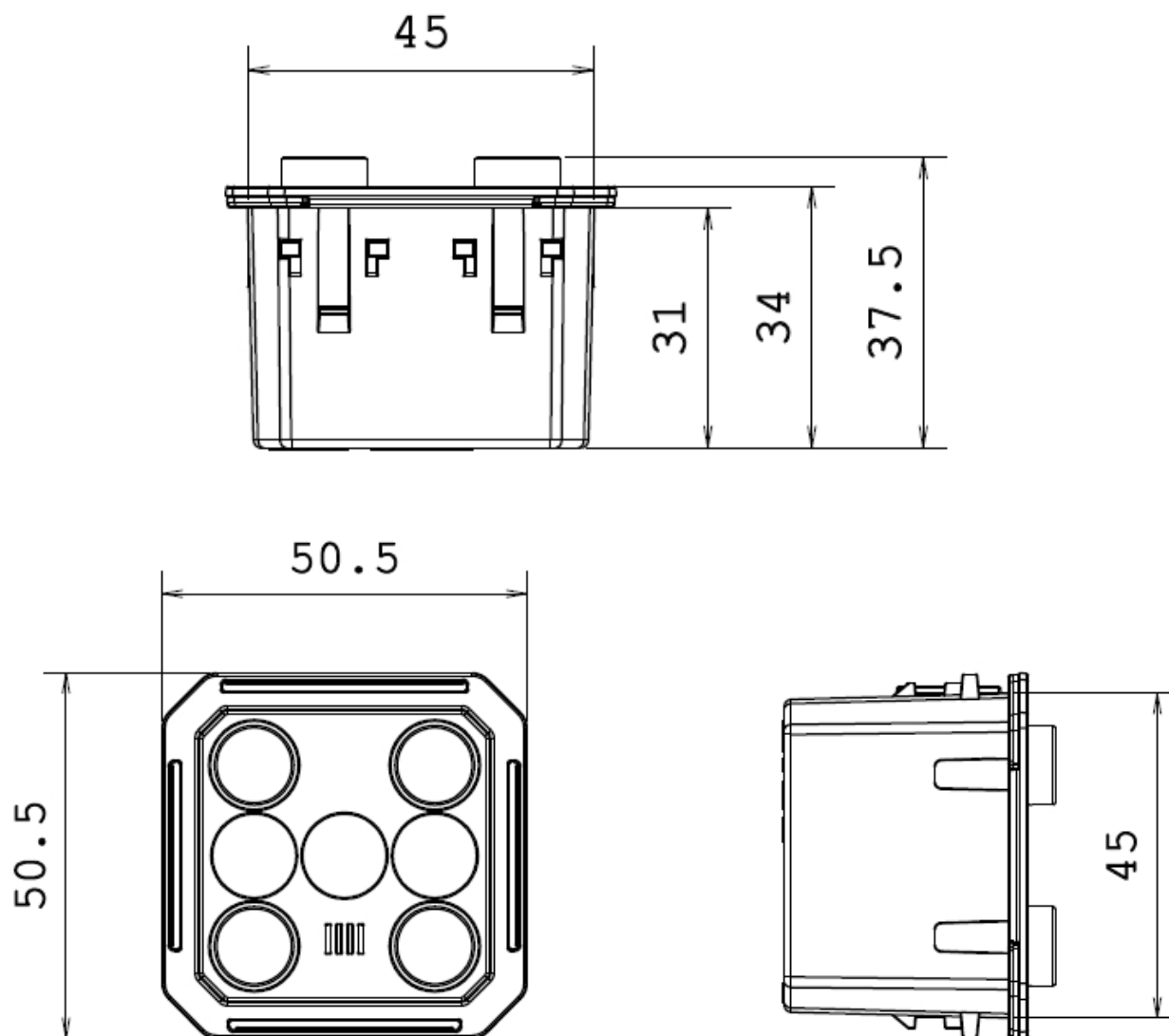
Figure 1 – Dimensions for EK-EZ2-TP-x
