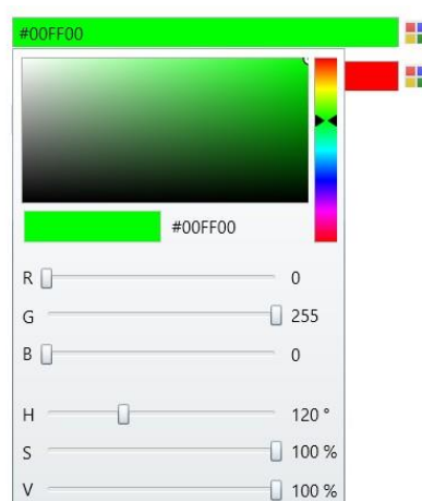
Figure 7 - Colour picker
