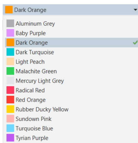
Figure 8 - Color palette
