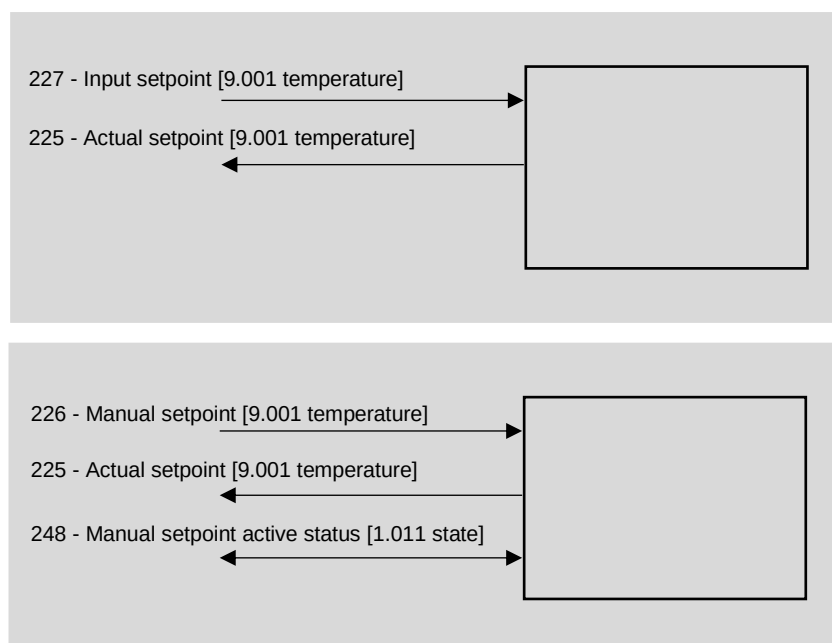
Figure 25 – Remote setpoint setting
