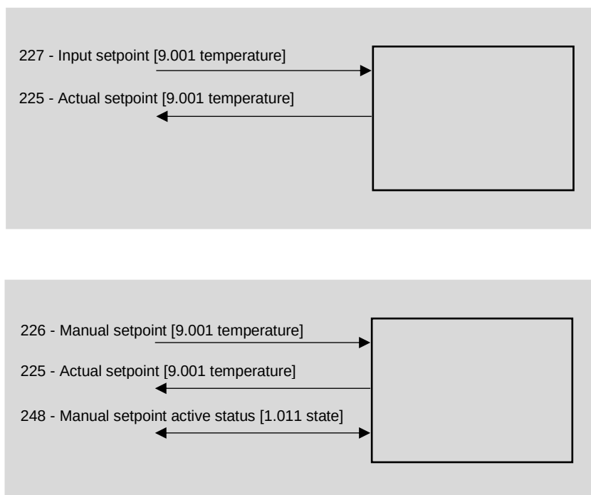
Figure 25 – Remote setpoint setting
