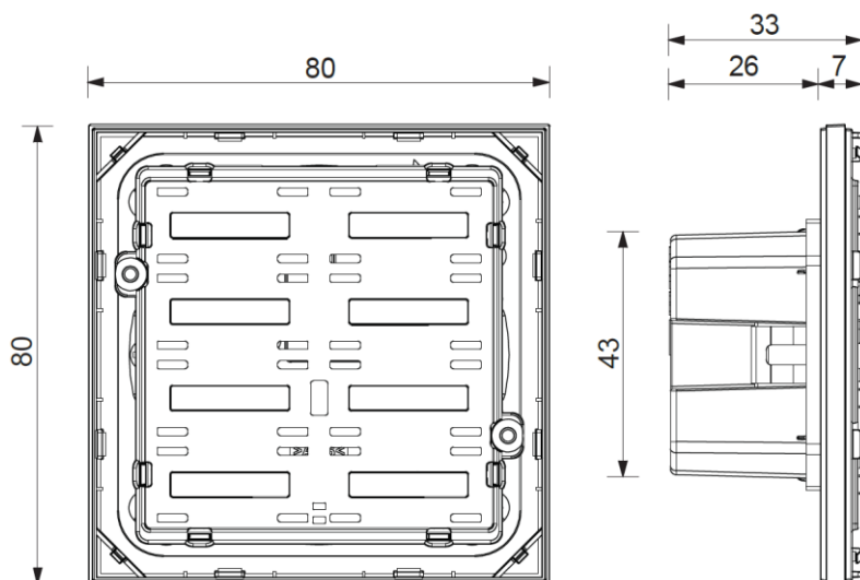
Figure 1 - EK-E2E-TP-4x, EK-E2E-TP-8 with square support
