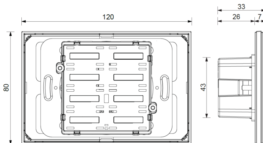
Figure 2 - EK-E2E-TP-8 with rectangular support
