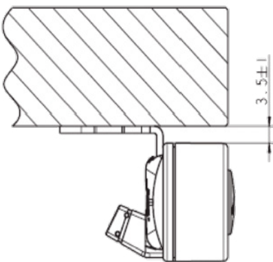
Example 2 (on request) The control is mounted with a 90° bracket and spaced (3.5 ± 1 mm) from the cabinet top
