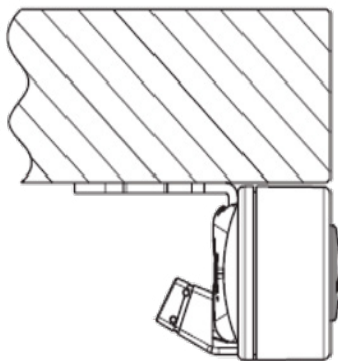
Example 1 (included in delivery) The control is mounted with a 90° bracket and positioned close to the cabinet top
