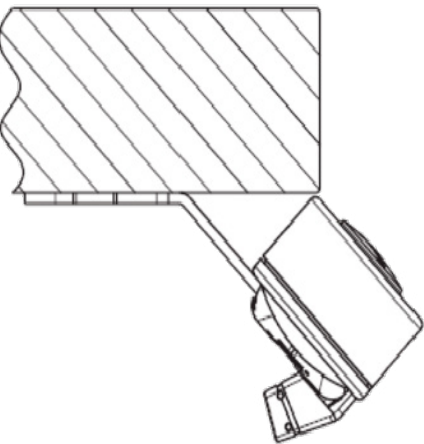
Example 3 (on request) The control is mounted with a 45° bracket and placed on the edge of the cabinet top
