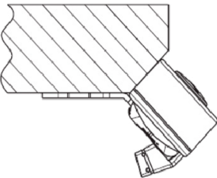
Example 2 (on request) The control is mounted with a 90° bracket and spaced (3.5 ± 1 mm) from the cabinet top
