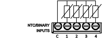
j Connection as 4 individually configurable inputs for passive temperature probes (NTC 10 kΩ at 25 °C).
