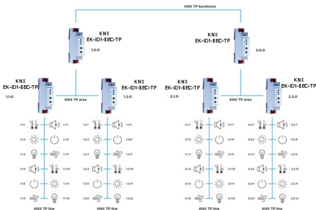
Figure 5 - Area coupler scheme
