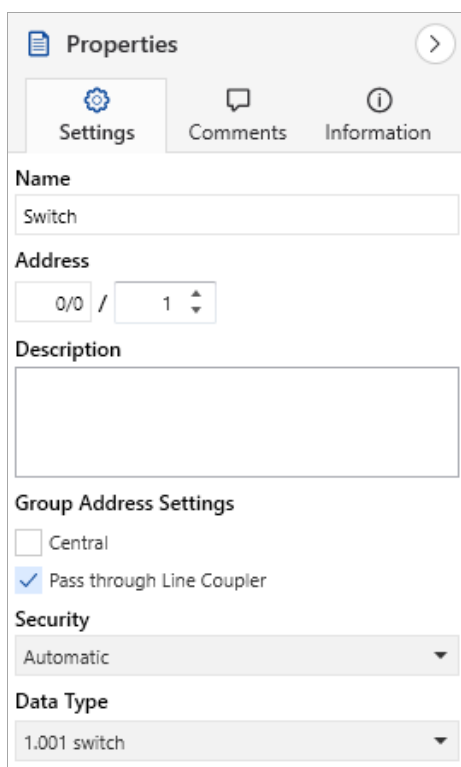
Figure 21 - Pass through Line Coupler setting
