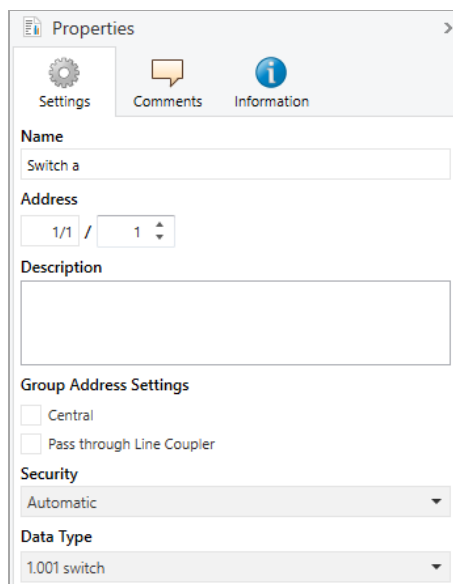
Figure 14 - Secure objects setting
