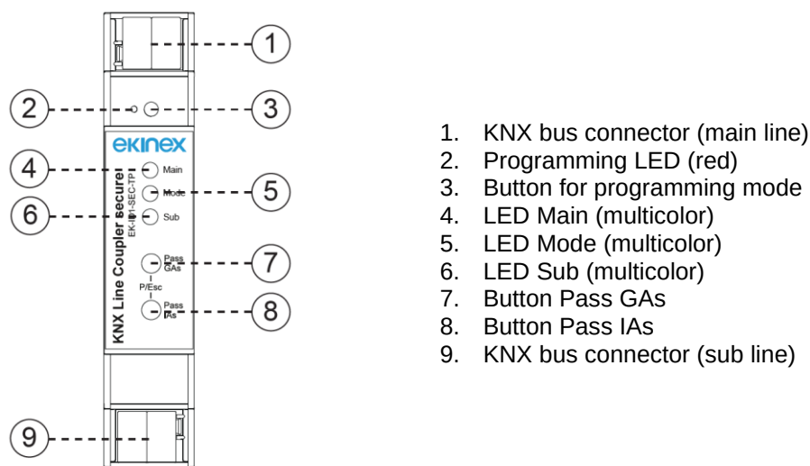
Figure 1 - EK-ID1-SEC-TP elements
