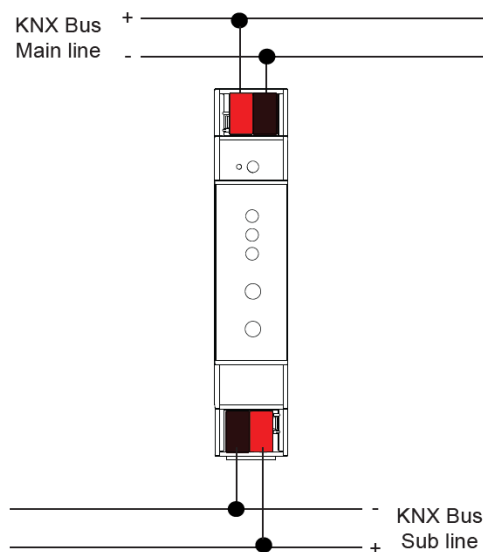
Figure 2 - Connections scheme
