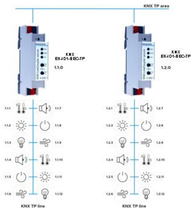
Figure 3 - Line coupler scheme
