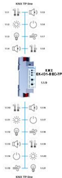
Figure 9 - Repeater scheme
